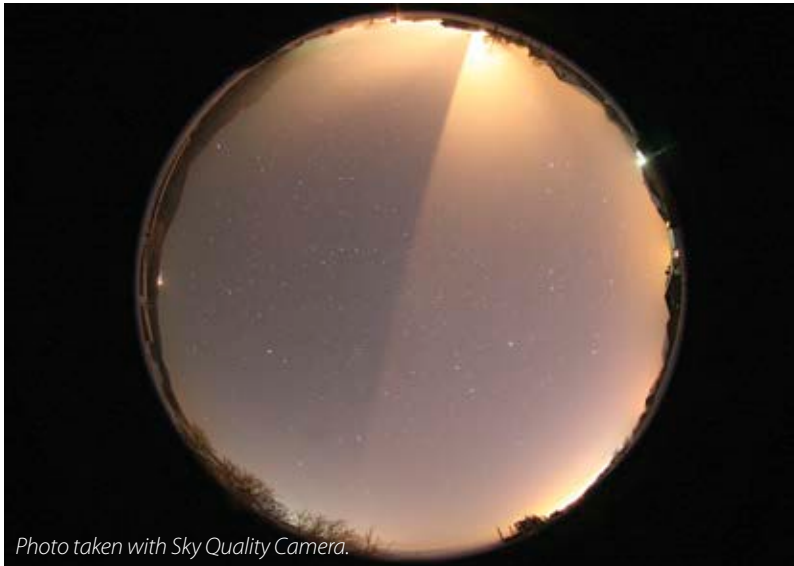
The photo taken with a Sky Quality Camera (fisheye) was taken a few hundred metres away from the church. It captures all 360 degrees of the sky. This is the standard method for measuring light pollution of the sky at a certain point. Software was used to analyse the levels of sky brightness. The results show a light polluted horizon and the sky surrounding the church where light beams spread in all directions. The belfry cuts the light beam from one of the reflectors and causes one half of the sky to be approximately 50% more illuminated (light polluted) than the other half. Even though this phenomenon is local, we should not forget that light spreads through the atmosphere more than 200 km away from the source and that light pollution at a certain location is the sum of all radiation in a circle with radius of 200 km. Improving the standard of lighting at only one site results in a measurable decrease in light pollution at a distance of several kilometres.
